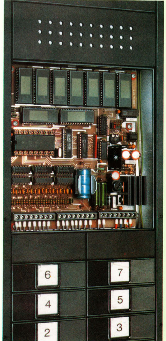
Standard kabin kumanda kasetimiz. Standard car operation panel.
